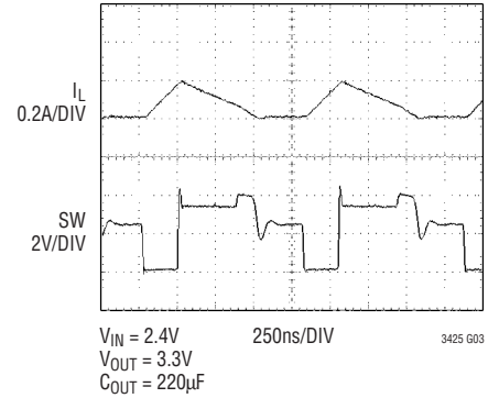
SW Pin and Inductor Current in Discontinuous Mode. Antiringing Circuit Eliminates High Frequency Ringing
